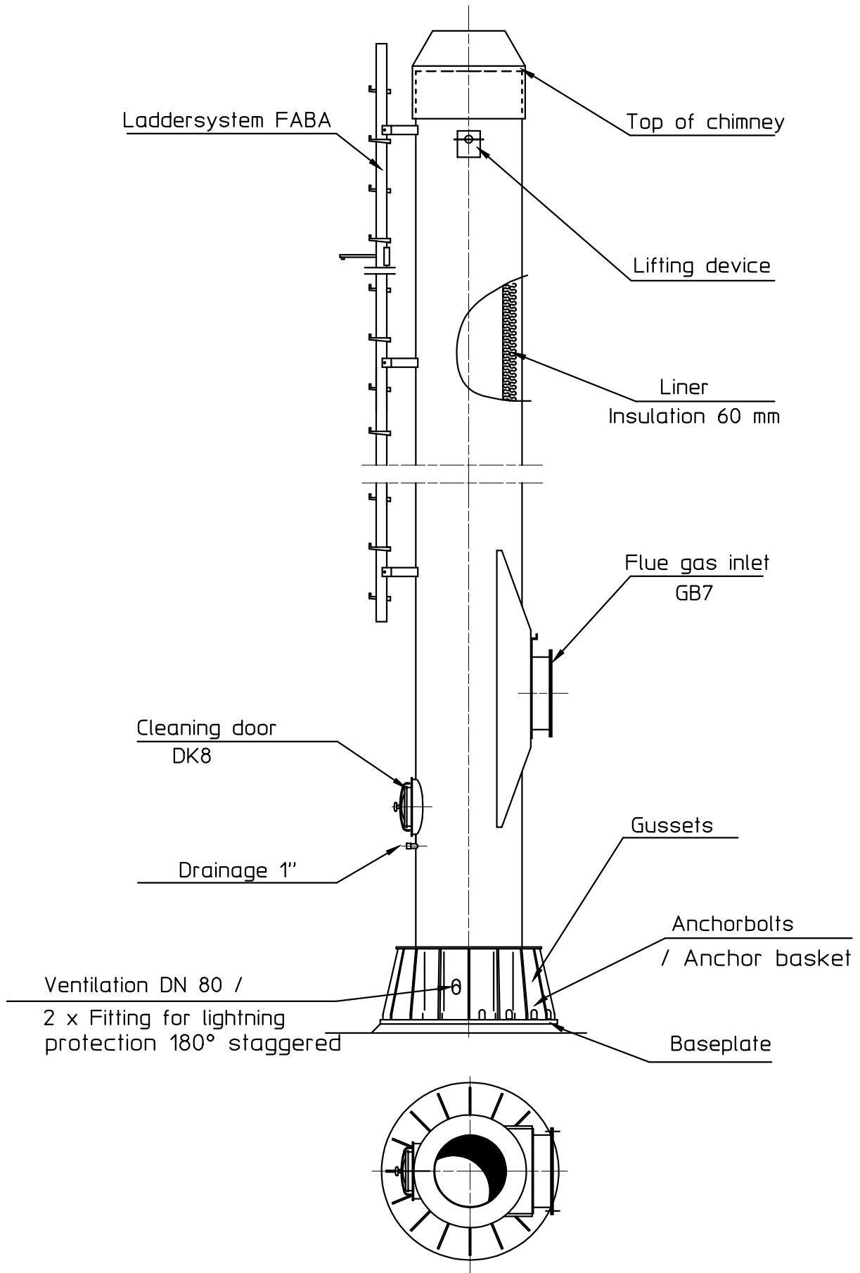
Steel chimney with one liner. GB1
