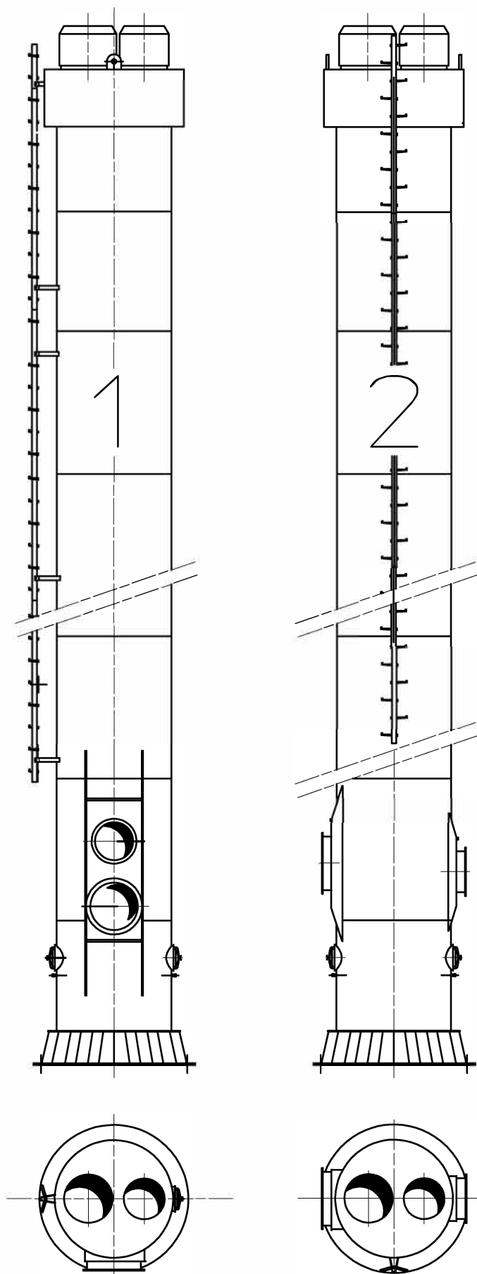
Chimney with two liners GB2
