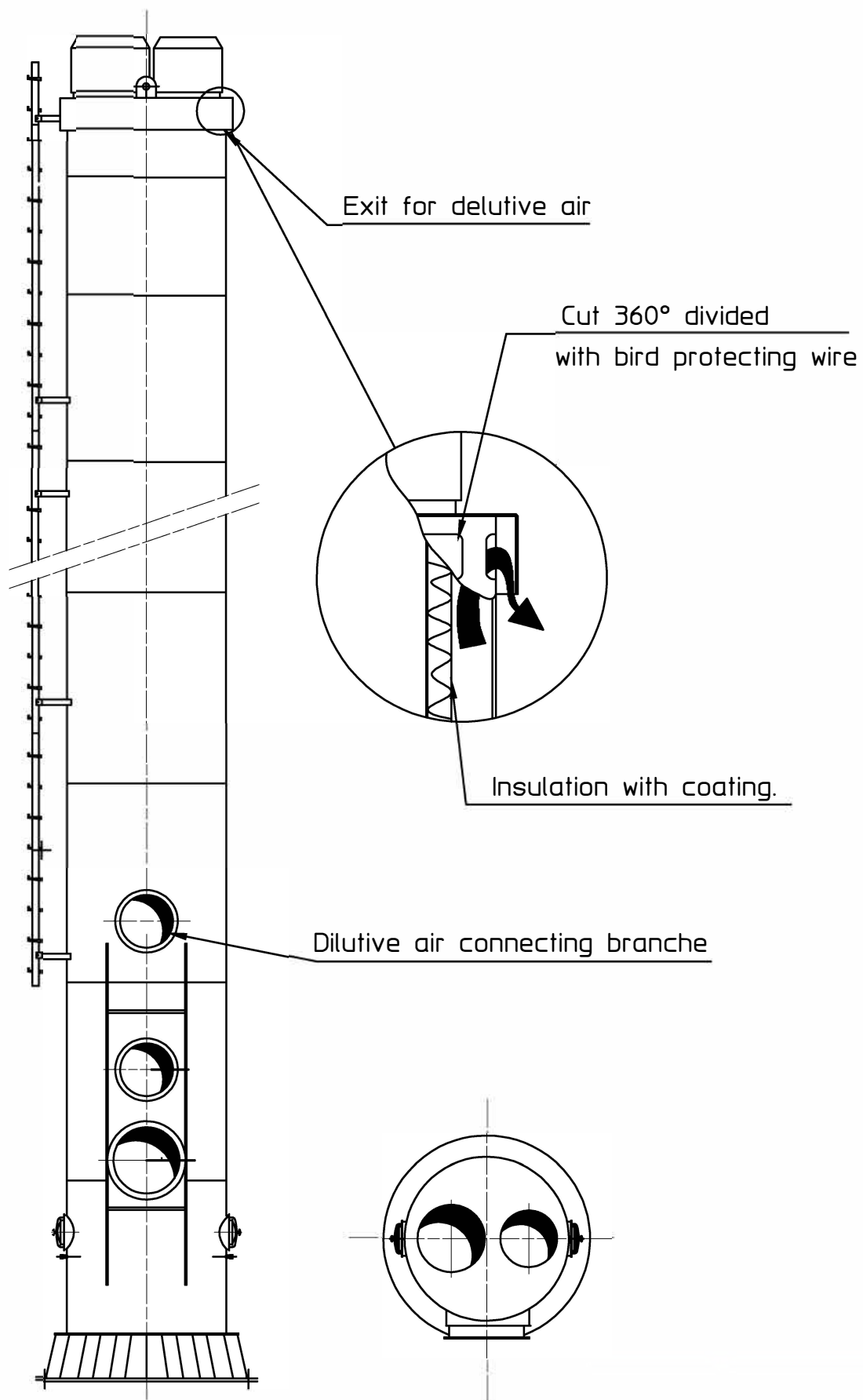
Steel chimney with integrated dilutive air GB6
